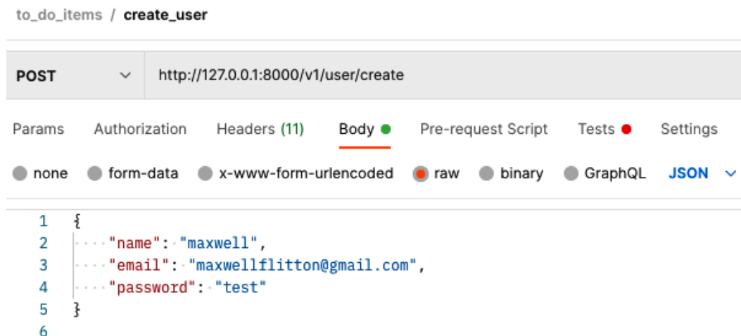
Figure 13.1 – Create user Postman request
