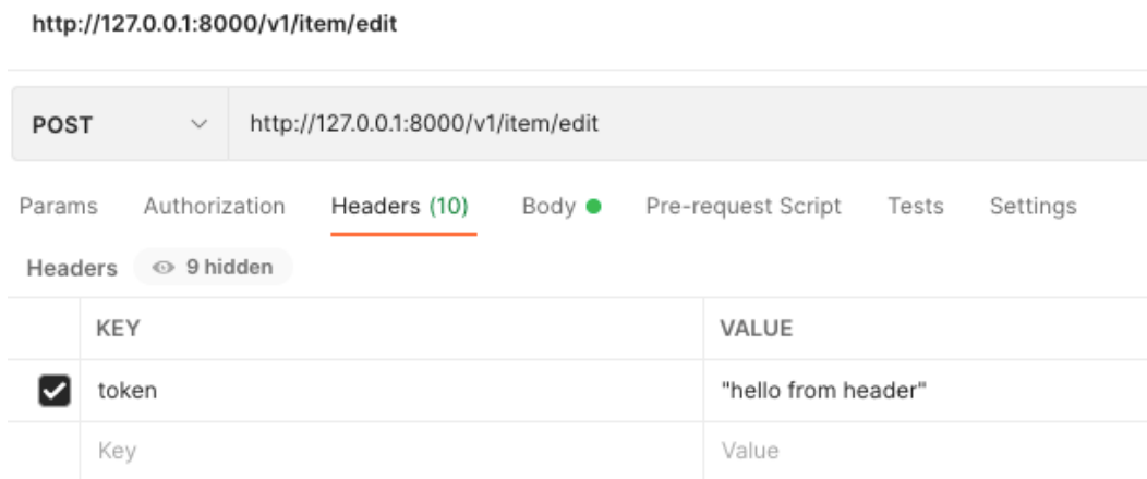
Figure 4.9 – Edit request in Postman with header
