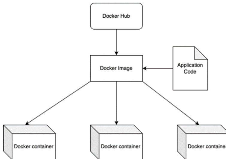
Figure 6.1 – Relationship between Docker images and containers
