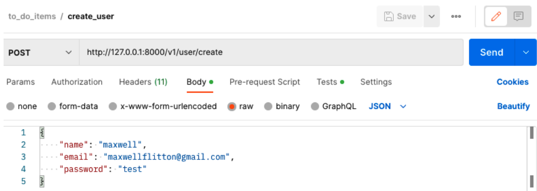
Figure 9.1 – Creating a new use Postman request
