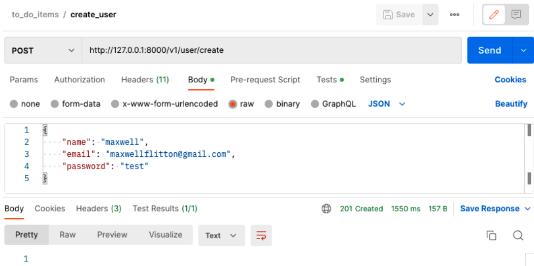
Figure 9.2 – Creating new use Postman response
