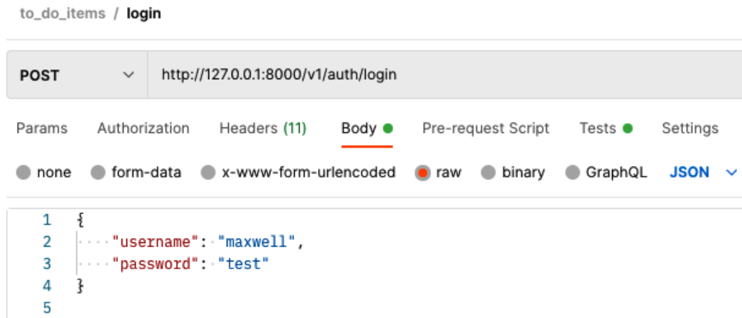
Figure 13.2 – Login Postman request
