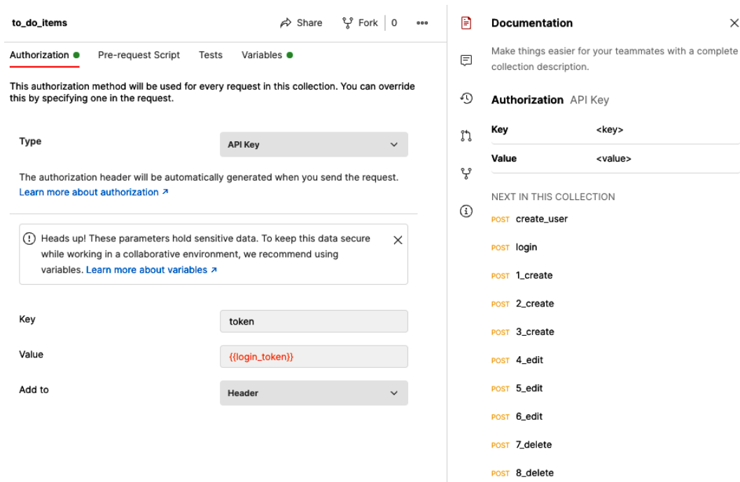
Figure 13.4 – Configuring authorization
