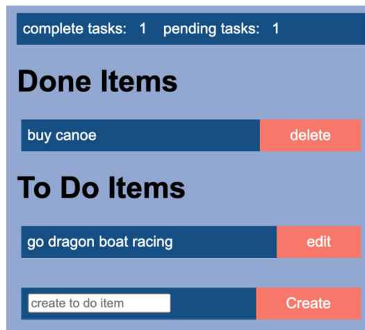
Figure 6.6 – Expected output
