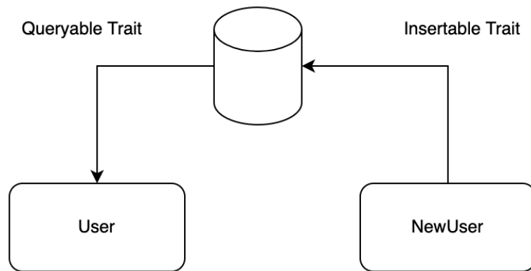
Figure 7.1 – Locking down data model structs with traits
