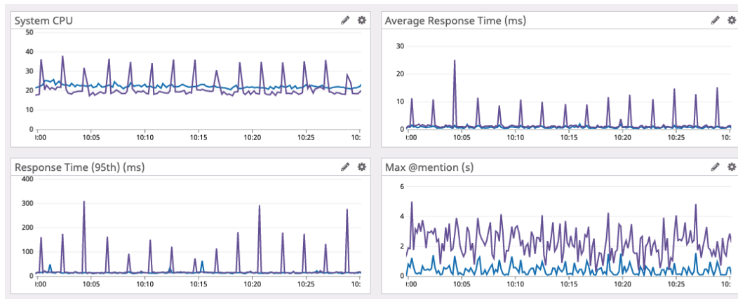
Figure 1.2 – Discord's findings => Golang is spikey and Rust is smooth (found at https://discord.com/blog/why-discord-is-switching-from-go-to-rust )
