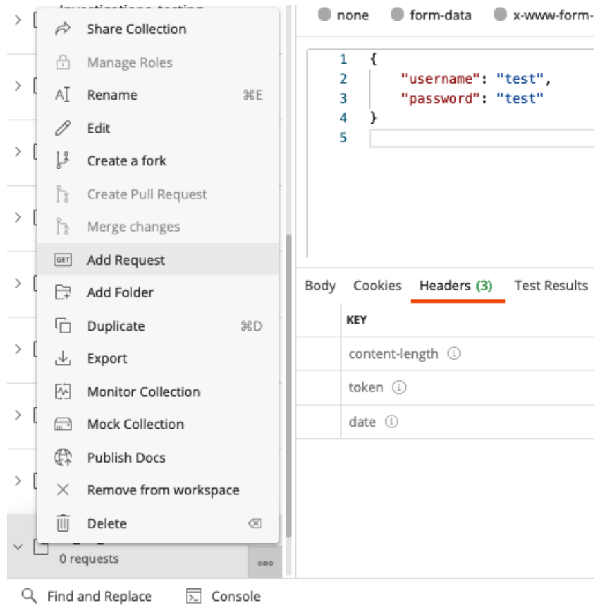
Figure 9.5 – Creating a new request for our Postman collection
