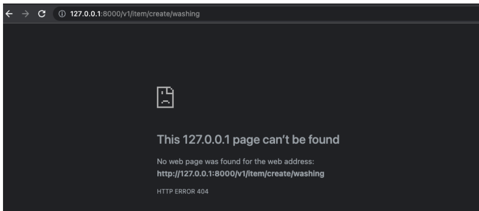
Figure 4.5 – Blocked method
