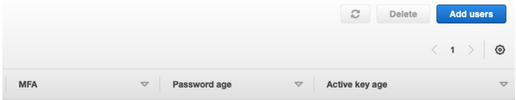
Figure 10.7 – Creating users
