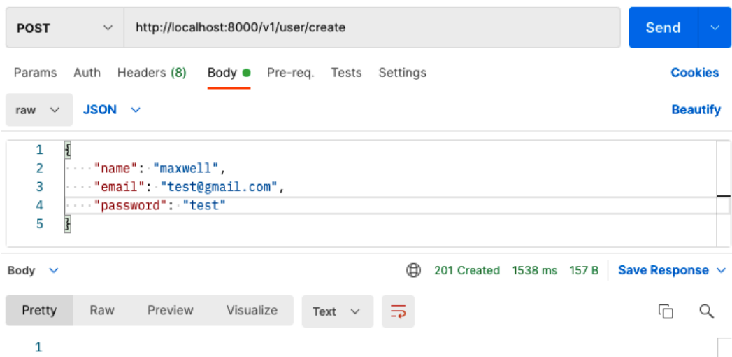
Figure 7.4 – Postman call to our create user endpoint
